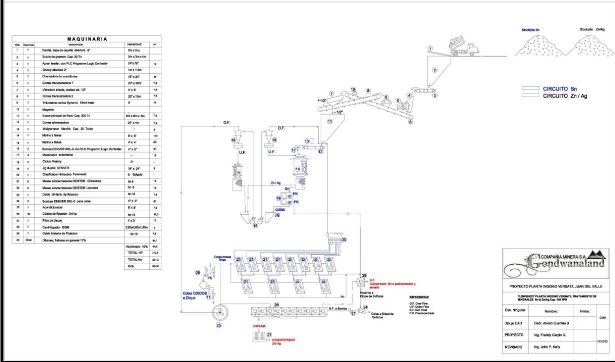
Figure 1 – 150tpd Treatment Plant Flowsheet for the San Pedrito Project
