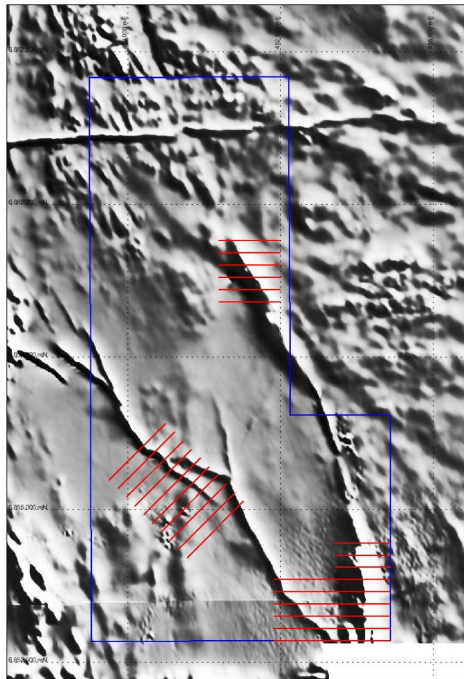
Figure 2: Proposed EM Survey Lines
